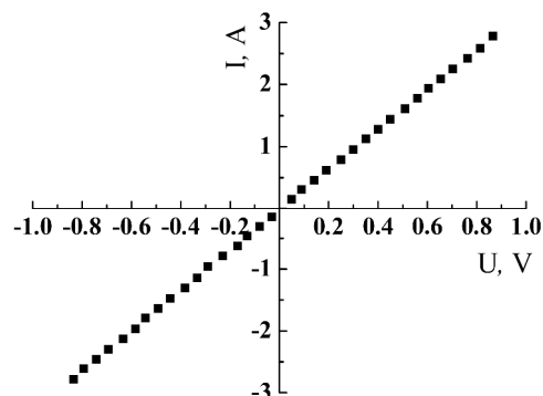
Fig. 1. The I-V characteristic of the In/TiO 2 contact.
