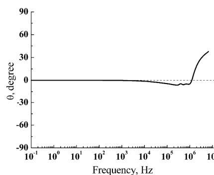
Fig. 2. The frequency dependence of the I-V phase shifting \theta(\nu) .
