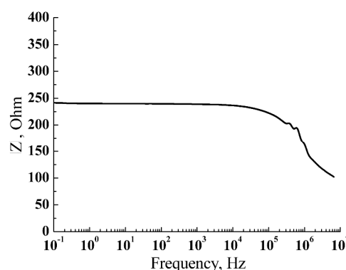
Fig. 3. The frequency dependence of the absolute value of impedance |Z(\nu)| of the Cu-Au/p + /p-CdTe/p + /Au-Cu structure.
